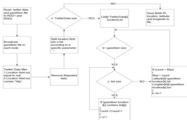
Figure 1. Workflow and algorithm to complete the geocoding procedure based on twitter user profile and gazetteer data
