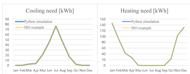
Figure 6. Comparison of energy needs with the assumptions explained in the ISO 13790:2008 (Annex J) for an office building room
