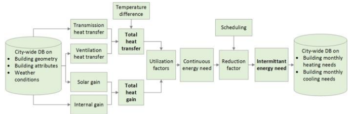
Figure 2. Implementation steps of the CityBEM monthly model for building energy need calculation
