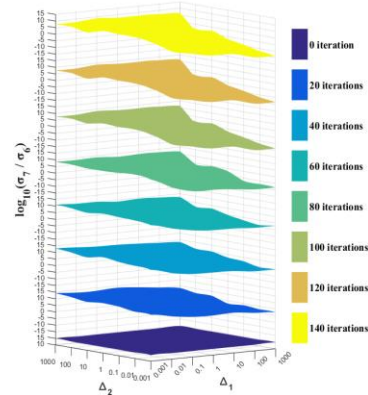
Figure 3. Rank constraints of various setting of \Delta_1, \Delta_2 and sp .
