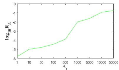
Figure 4. Block rotation constraint of various settings on \Delta_1 .
