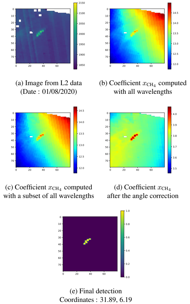
Figure 9. On all images, pixels in white are discarded pixels (cloudy for example). In (a), the L2 data with a methane plume in the middle of the image. In the other figures, the evolution of the coefficient x_{CH_4} at each step of the algorithm.
