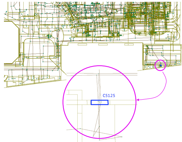
Figure 10. One of the many examples where dataset LWM has issues with the dual nodes. Cell “C5125” has 3 nodes inside, but none of them are linked by the cell (which has as a dual a non-existent node).
