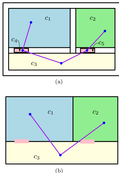
Figure 2. Two ways to model cells in an IndoorGML model. (a) 5 cells are present since doors (pink cells) are explicitly modelled. (b) The doors are not cells, their presence can be inferred by the fact that the navigation graph has an edge between 2 cells.
