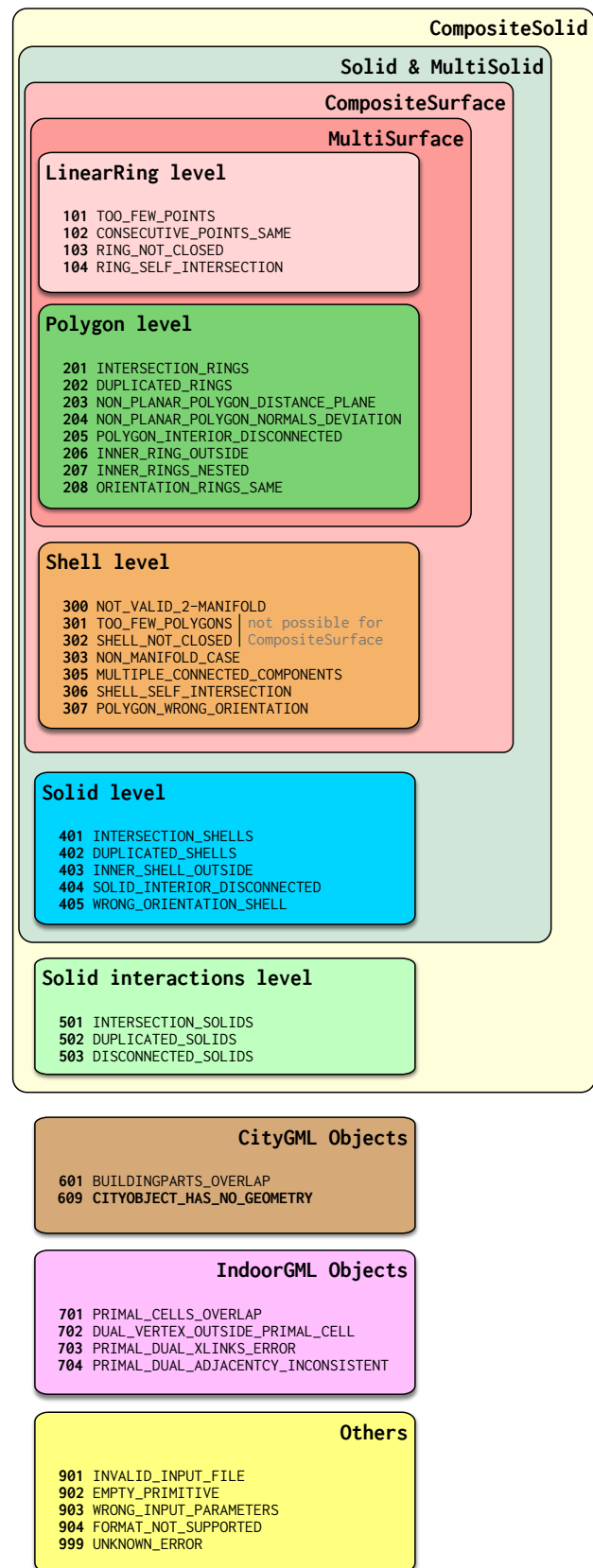
Figure 6. The 37 error codes of val3dity.
