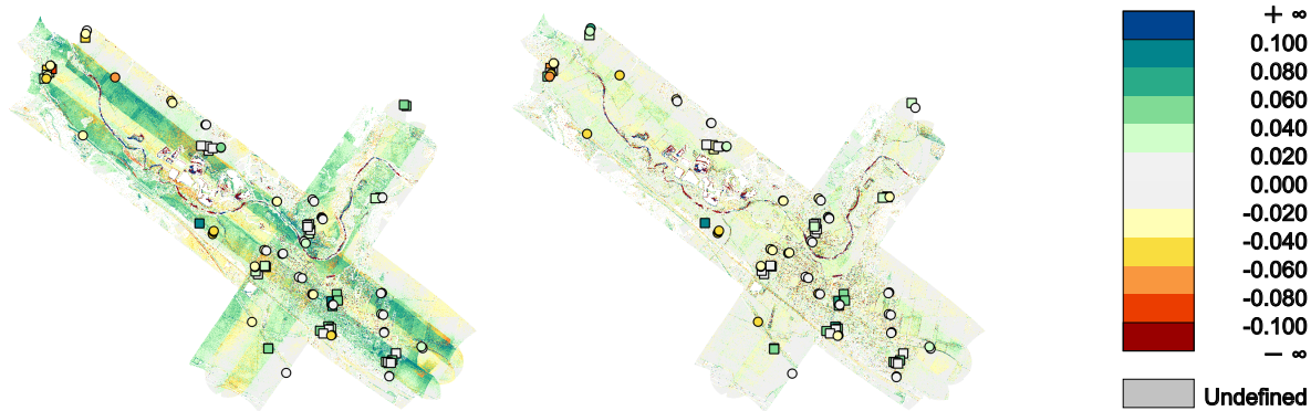
Figure 4. Strip height differences [m] after standard strip adjustment with RiPRECISION (left) and GNSS/INS/LiDAR-integrated adjustment (right). Overlaid on the strip differences are normal distances to ground truth targets of two types: check points on horizontal surfaces on the ground (circles) and on sloped rooftops (squares), after application of the estimated datum shifts.
