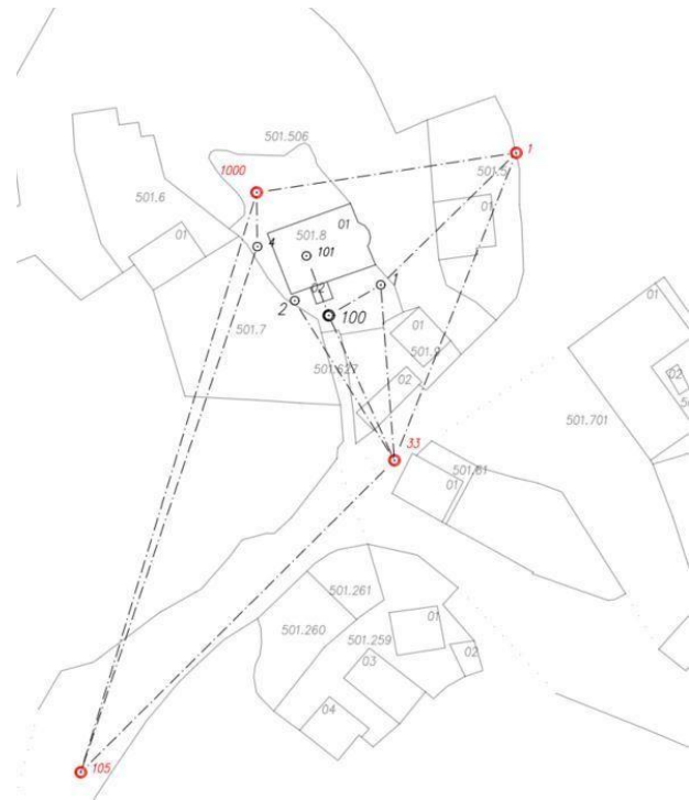
Figure 2. Spatial distribution of existing and newly established control points around and inside the Church of St. Petka.
