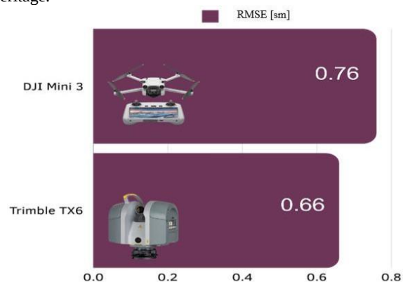
Figure 11. RMSE values in cm derived from the comparison of control distances for the Church of St. Petka.
