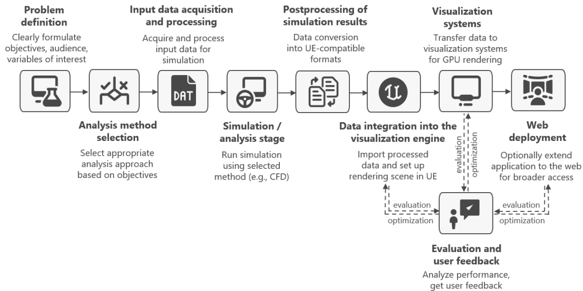
Figure 1. Workflow for smart cities visualizations.
