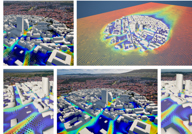
Figure 2. Direct representation of raw CFD data at the computational mesh nodes. Views of wind velocity distribution at pedestrian height (lower values shown in blue, higher - in red).
