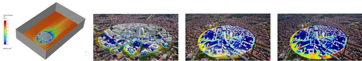
Figure 7. Visualizations of the velocity field in the investigated region via (left to right): 1/ ANSYS Fluent; 2/ Visualization of raw point data in UE; 3/ Unrefined Point-Based Velocity Visualizer; 4/ Refined Point-Based Velocity Visualizer
