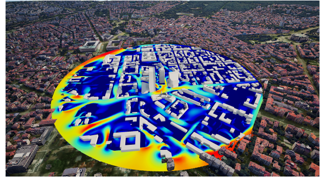
Figure 4. Refined Point-Based Velocity Visualizer. Visualization of pedestrian-level wind speed
