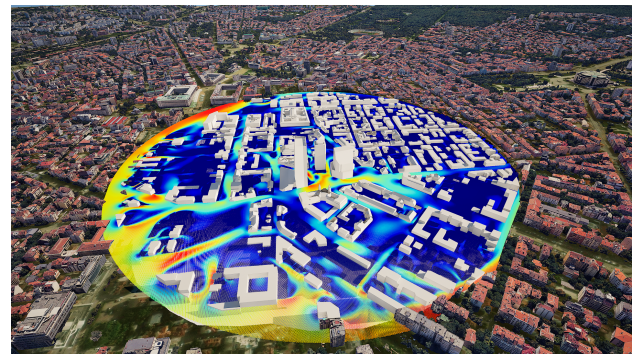
Figure 3. Point-Based Velocity Visualizer without refinement. Visualization of pedestrian-level wind speed.
