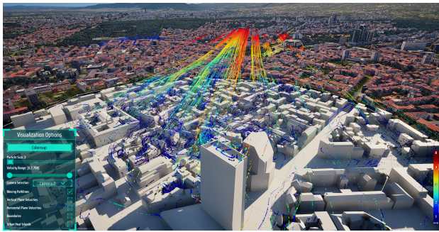
Figure 5. Streamlines Visualizer point of view 1. Wind flow paths representation
